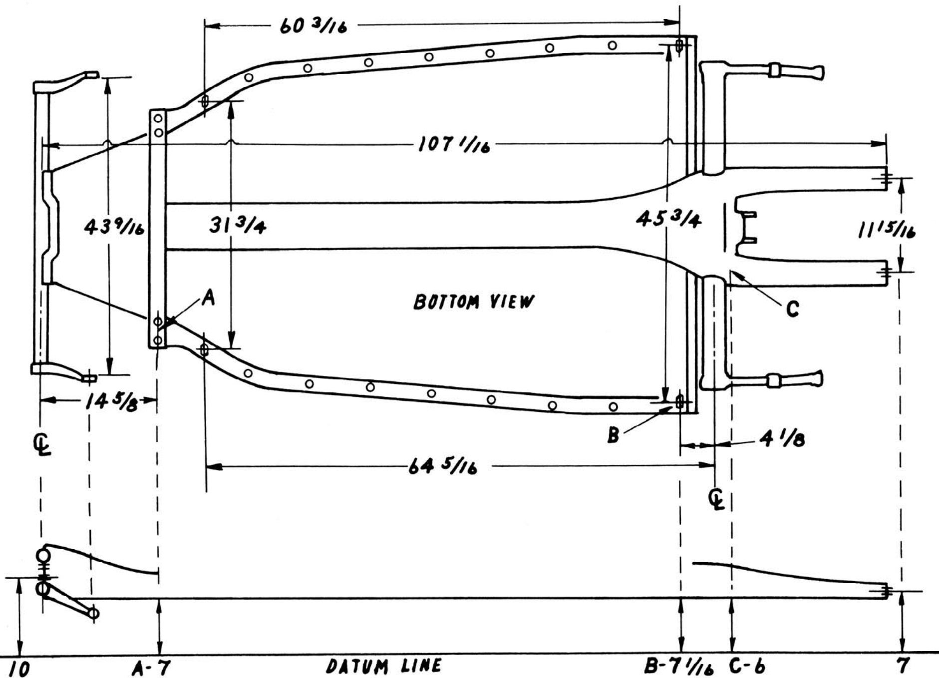
Volkswagon Types 11-14-15
