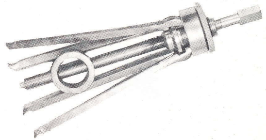
New rear axle bearing puller, including ring to adapt for front axle bearing.
