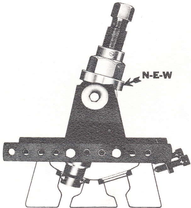
Valve seat puller
