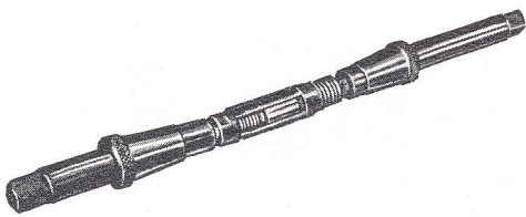
King pin bushing reamer, sedan, 18-21mm L. Spare blades, 18-21mm A. King pin bushing reamer, transporter, 21-24.5mm AL. Spare blades, 21-24.5mm
