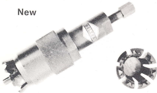
FANTASTIC rear axle bearing puller: guaranteed
