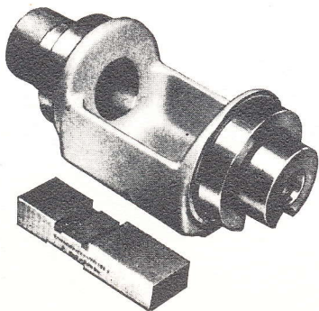
Transmission case mandrel gage, 40hp, in wood box
