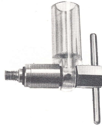
Float level gage, Zenith
