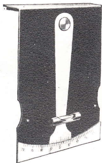
Caster and camber protractor L. Replacement float bubble
