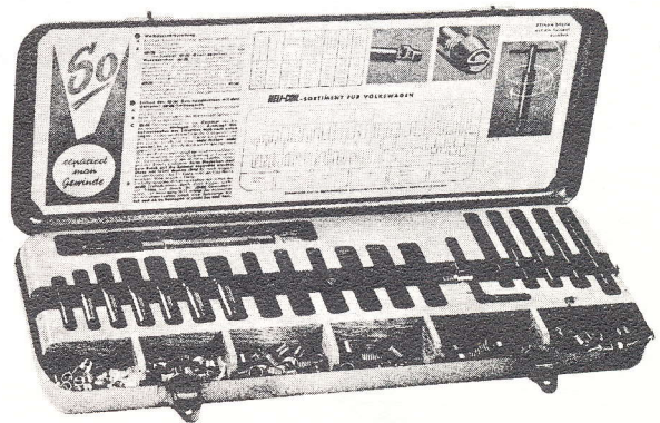
Metric Heli-Coil set: 6 x 1, 7 x 1, 8 x 1.25, 10 x 1.5, 12 x 1.5 & 14 x 1.5mm
