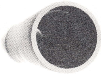
Tube for removing transmission case bearings, lower torsion arm ball joint, distributor drive gear, crankshaft timing gear etc.
