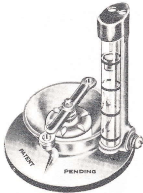
Carburetor synchronizer for 1500S and Porsche (P75)
