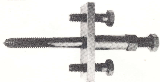
Fuel pump spacer puller
