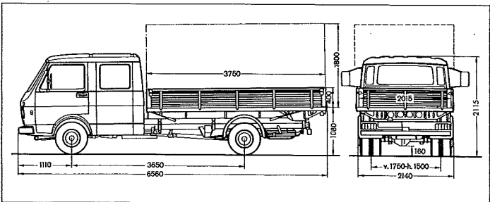
Double-cab pick-up LT 40/45/50/55
