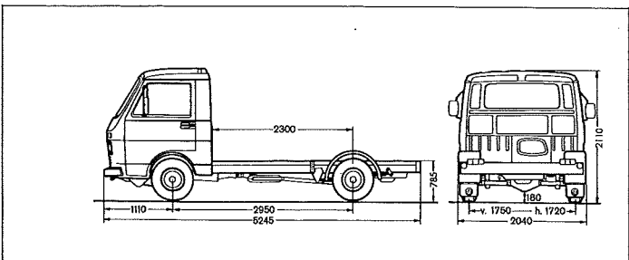
Chassis with cab LT 28/31/35
