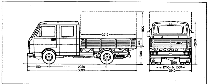
Double-cab pick-up LT 40/45/50/55
