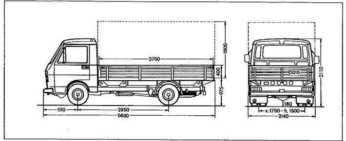
Pick-up LT 35
