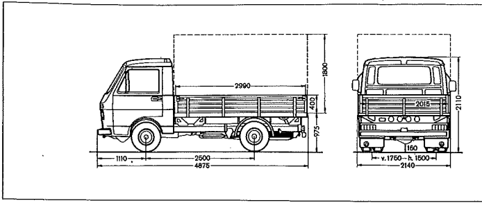
Pick-up LT 35
