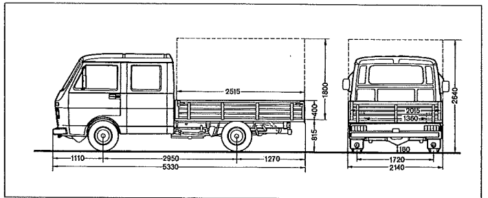
Low-loader with double-cab LT 28/31/35
