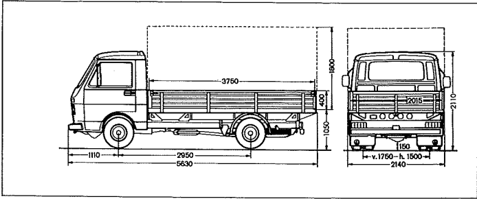
Pick-up LT 40/45/50/55
