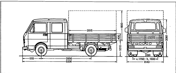
Double-cab pick-up LT 35
