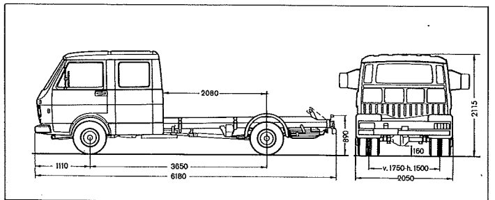
Chassis with double cab LT 40/45/50/55
