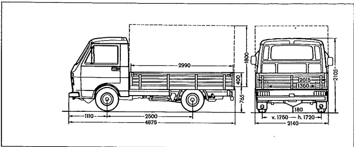
Low-loader LT 28/31/35
