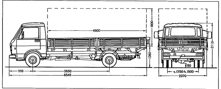
Pick-up LT 40/45/50/55
