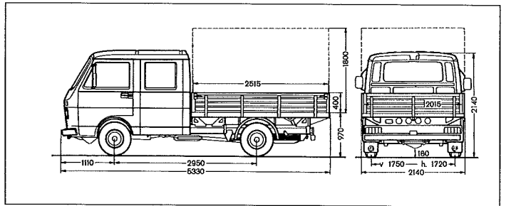
Double-cab pick-up LT 28/31/35
