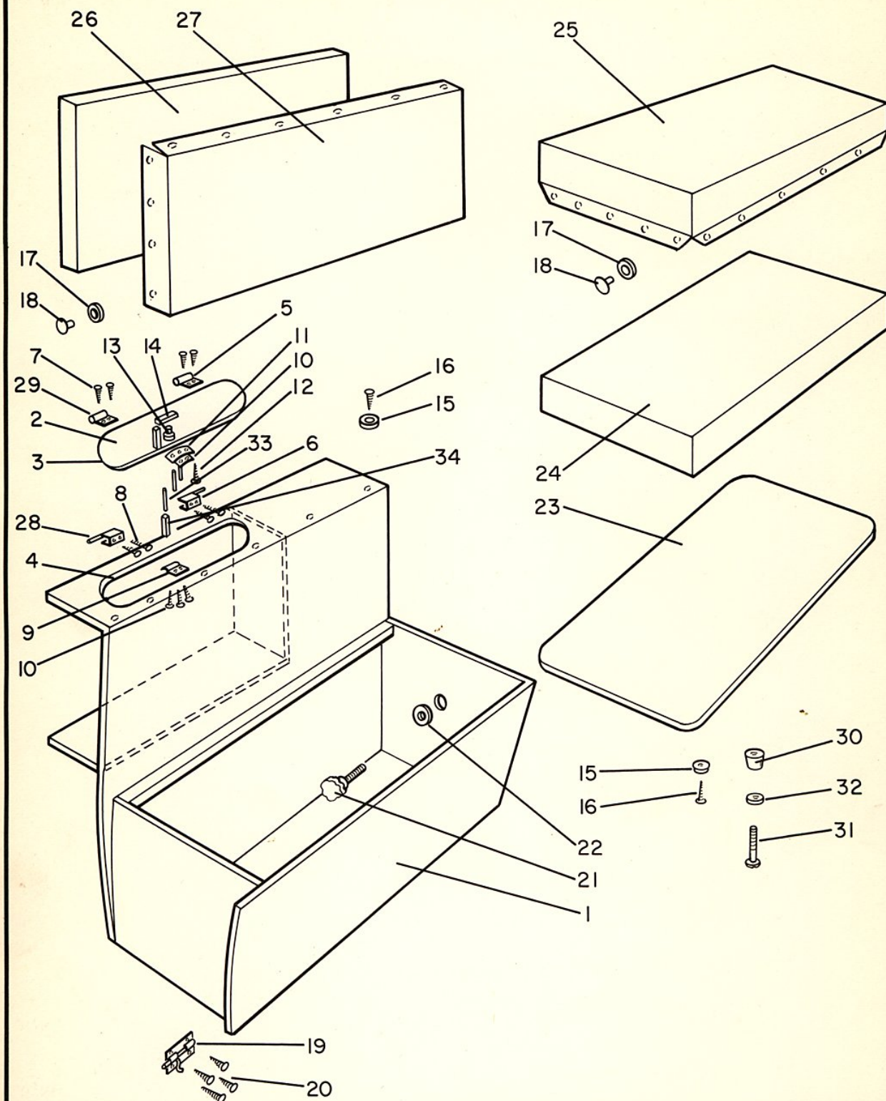
SEAT BOX AND CUSHION MODEL 216001
