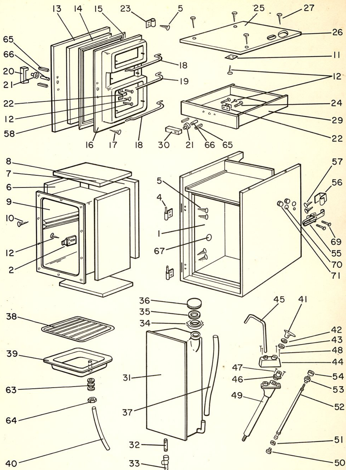
ICE BOX CABINET MODEL 216001
