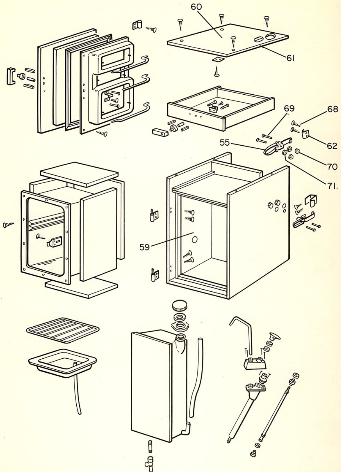
ICE BOX CABINET MODEL 216002
