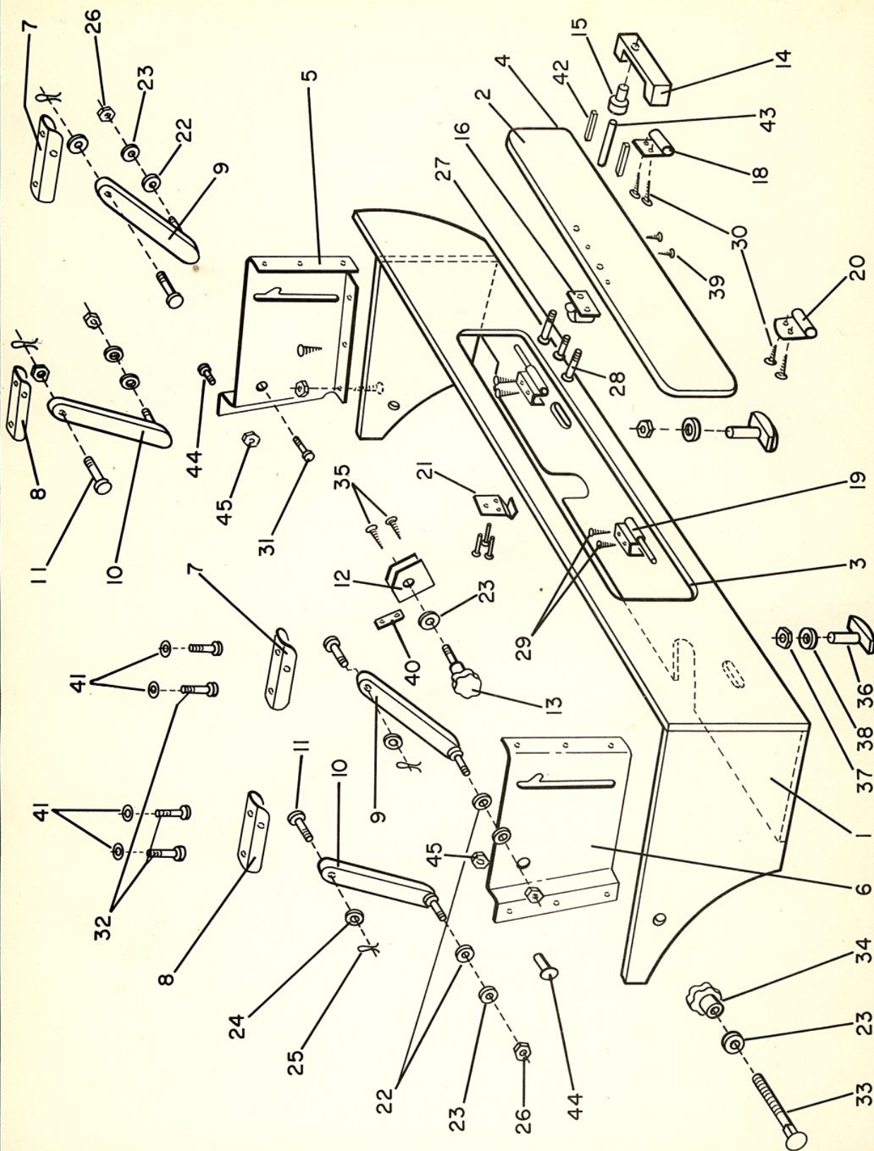
SEAT BOX REAR
