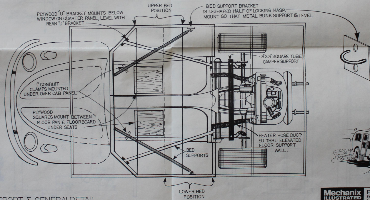
BED SUPPORT & GENERAL DETAIL SCALE 1"=1'-0"
